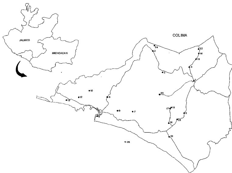
FIG. 1. Areas of greatest species diversity of Rhopalocera in the state of Colima. Major highways in Colima are indicated on the map by solid lines. Numbers correspond to localities listed in Table 2, the 25 localities in the state with the greatest numbers of recorded species (#1 = greatest; #25 = fewest recorded species; #25, Revillagigedo Islands are not shown on the map). Smaller map shows the positions of Jalisco, Colima and Michoacán in western Mexico.
